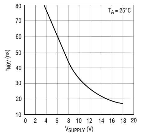
Break-Before-Make Time, t_{NOV} , vs Supply Voltage
